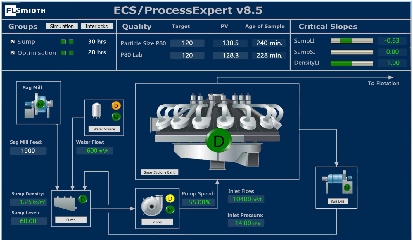
FLSmidth Process Control System showing grinding circuit “island of optimization” and some of the input parameters that are used to develop a comprehensive control strategy to maximize throughput and profitability in the comminution circuit.
