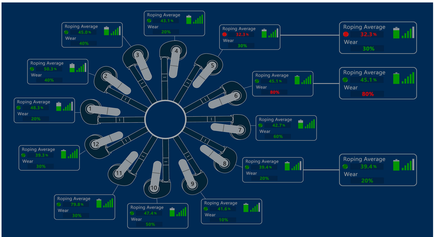
FLSmidth SmartCyclone display screen showing wireless roping sensor and wireless wear sensor output values. Operators can set warning and alarm values for these parameters.
